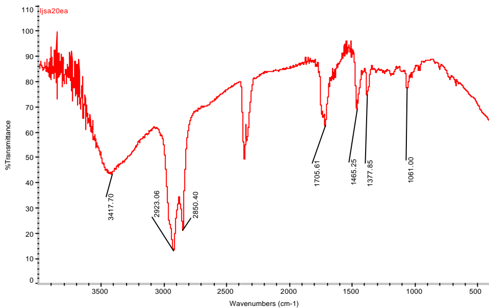
圖 10 : IR spectrum of compound IV
